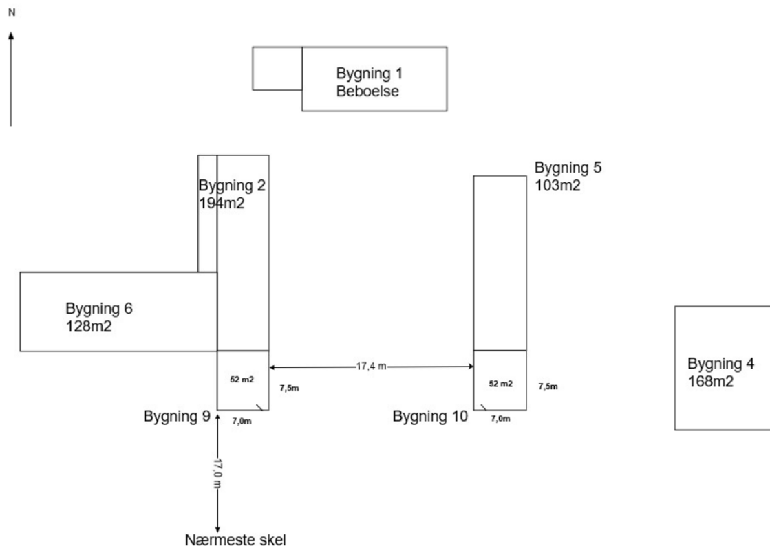
Situationsplan
