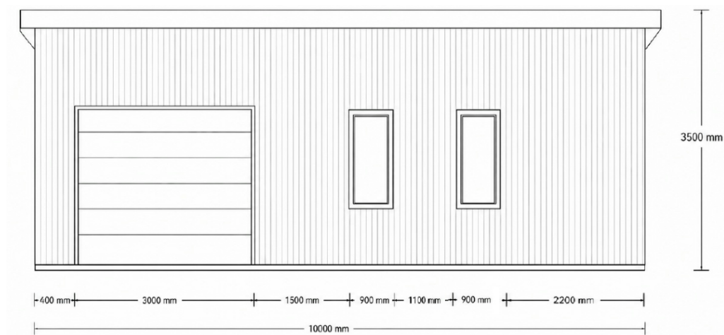
Figur 2 Facade mod vest
