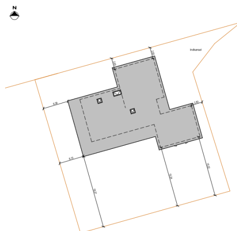
Situationsplan
